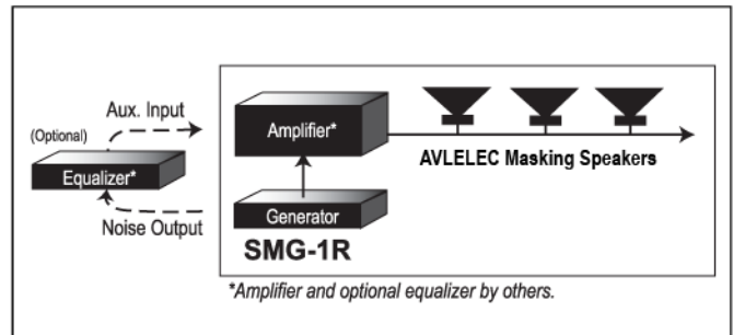
Typical Configuration Sound Masking Generator Models SMG-1R, SMG-1
